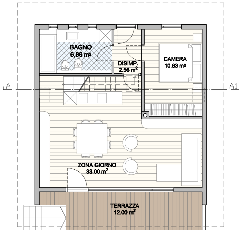
PIANO TERRA 51.60 m 2 scala 1:100
